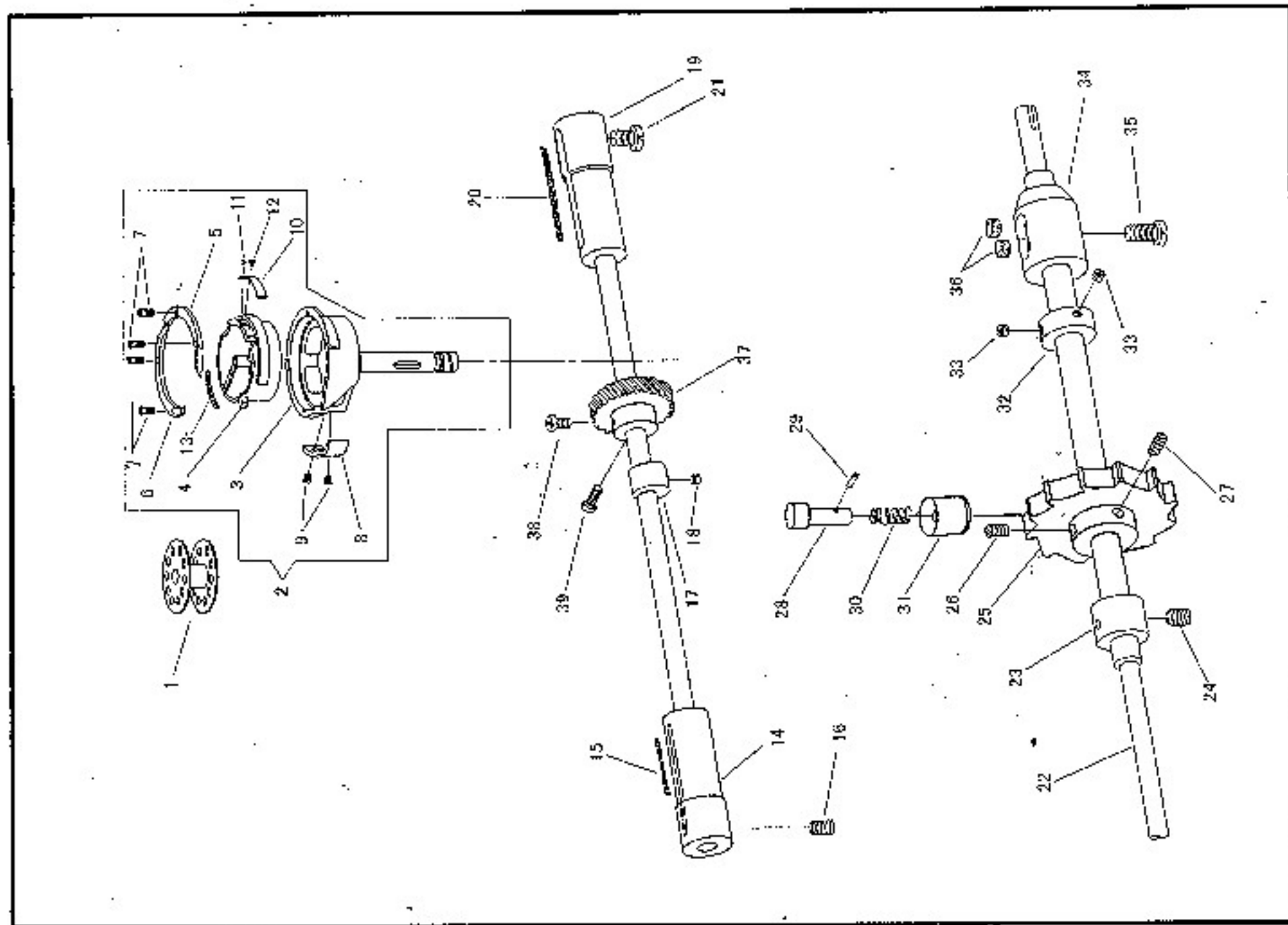
カム(右)、下軸 HOOK (RIGHT), HOOK DRIVING SHAFT
