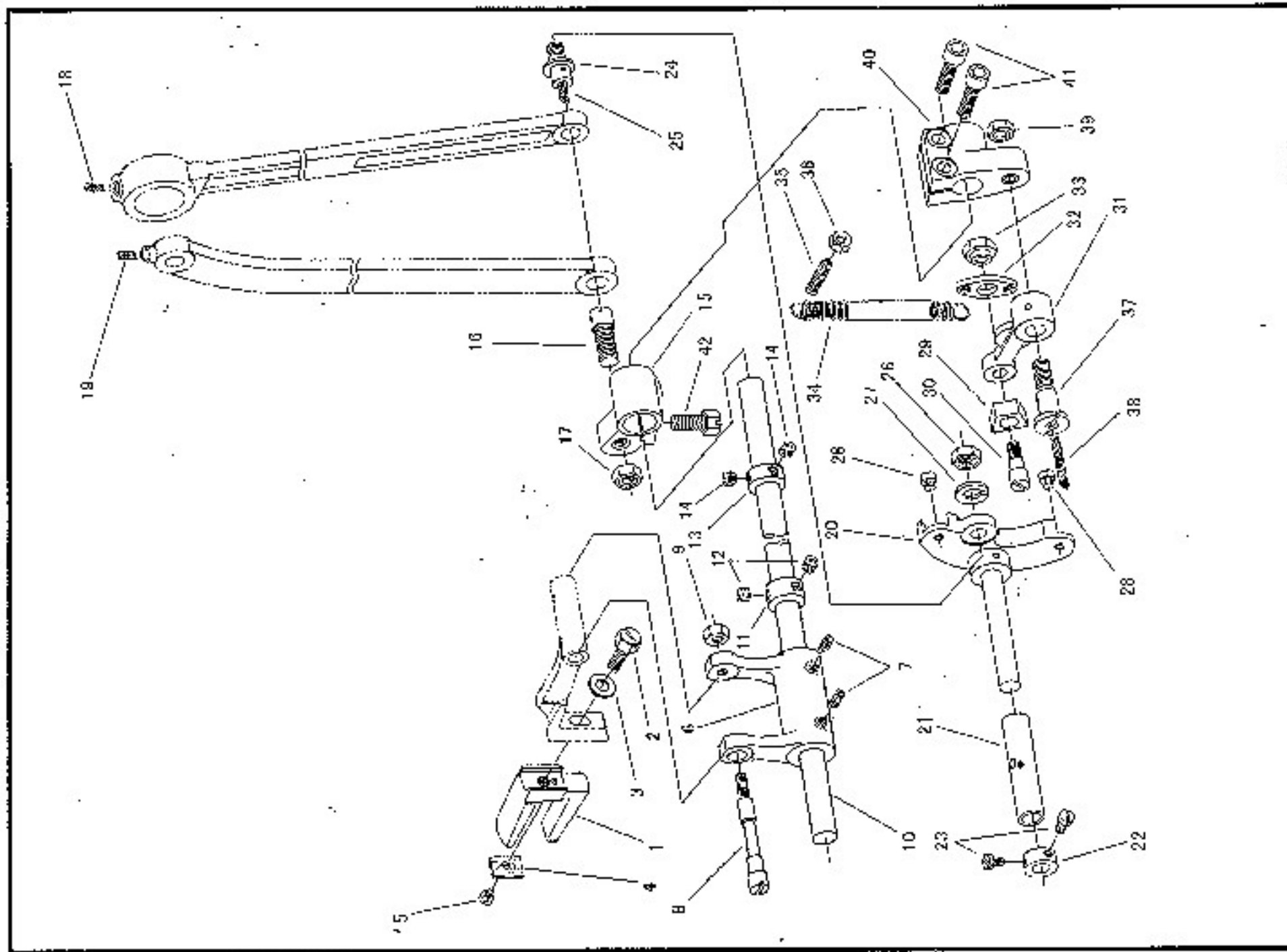
送り歯、送り軸 FEED DOG, FEED DRIVING ROCK SHAFT
